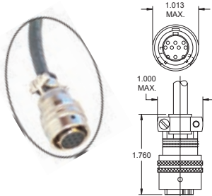
10 Pin Straight Cable (951, 952, & 953 Connector Option E)
