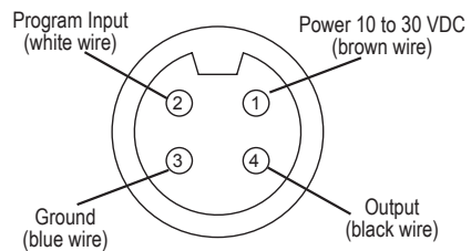
Connector View
