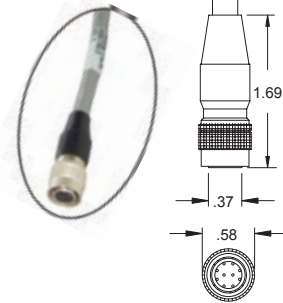
10 Pin Straight Cable (955DQ Connector Option H) (OBSOLETE)
