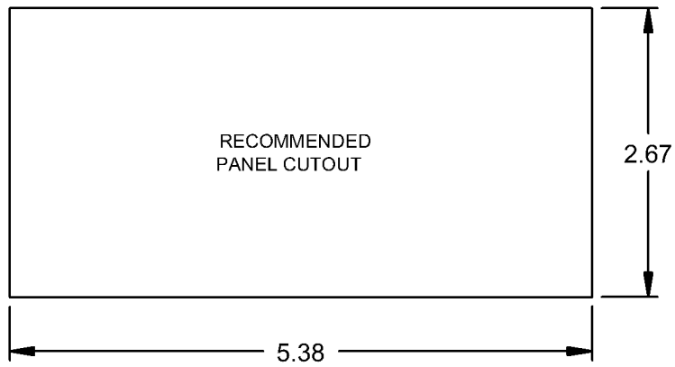
Figure 3-1 Dimensional Drawing Drawing E0232200
