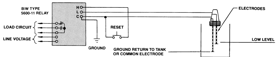
DIAGRAM C: LOW LEVEL ALARM OR CUT OFF – 5600-11 DIRECT OPERATION – WITH LOCK-IN & RESET PUSHBUTTON
