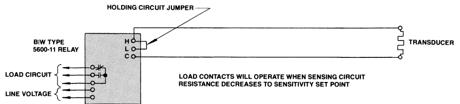
DIAGRAM D: CONTROL FROM RESISTIVE TRANSDUCER – 5600-11 DIRECT OPERATION – LOAD ACTUATION ON DECREASING RESISTANCE
