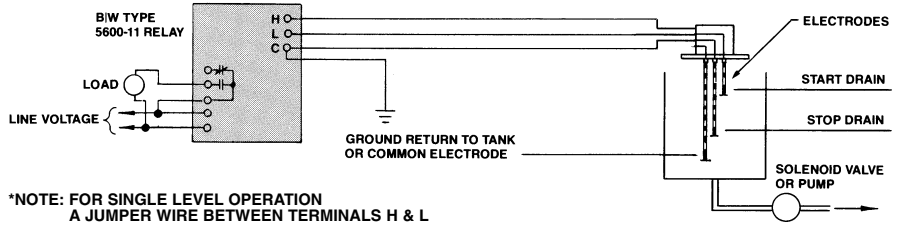
DIAGRAM B: PUMP UP CONTROL – 5600-12 INVERSE OPERATION
