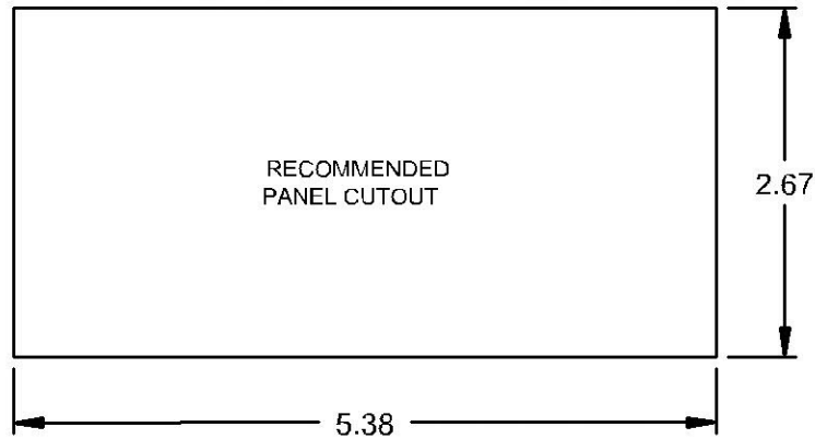
Figure 3-1 Dimensional Drawing
