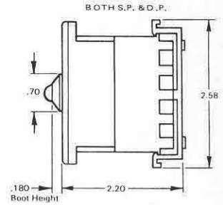
PLUG-IN SNAP SWITCH WITH PLUG-IN SOCKET ASSEMBLY AND PLUNGER BOOT OPTION
