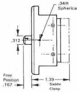
SNAP SWITCH WITH STANDARD "DO" OPERATOR AND SADDLE CLAMP OPTION (S.P.D.T. ONLY)
