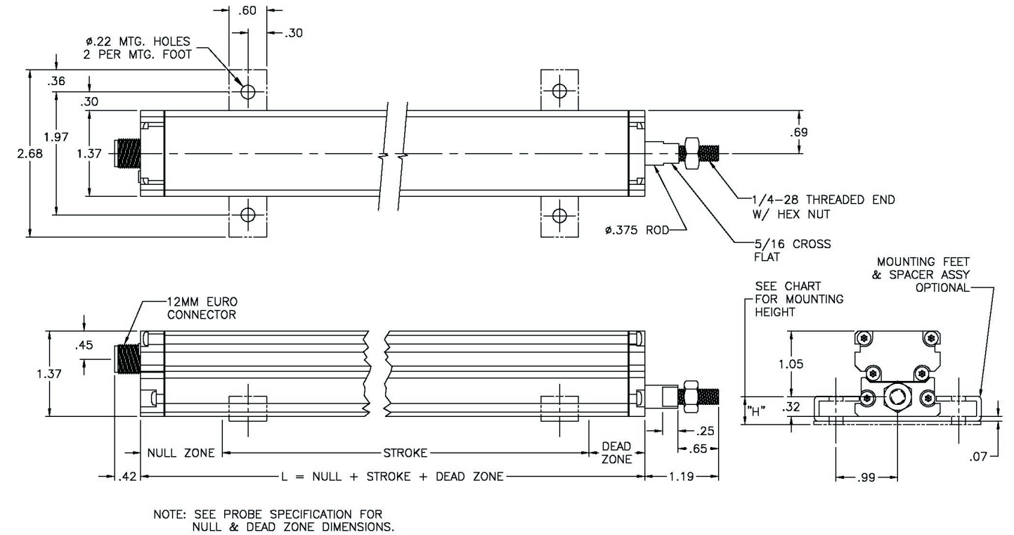
Optional Rod End. Part # 04-570256
