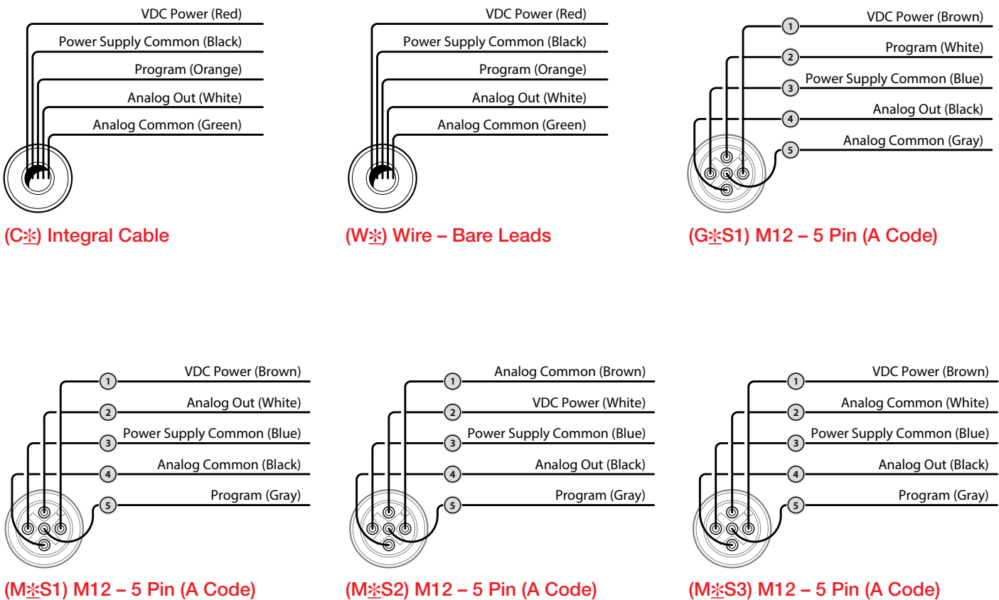
Figure 3-2: Pinouts and Wiring
